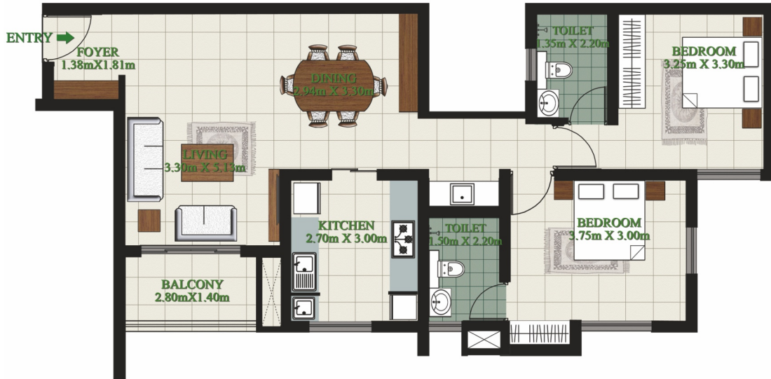
TYPE D & F (2 BHK) 1150 Sq.Ft. 2 nd Floor to 9 th Floor
